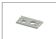
KT214/SF Adapter plate with stay bolts and screws H30 series.
